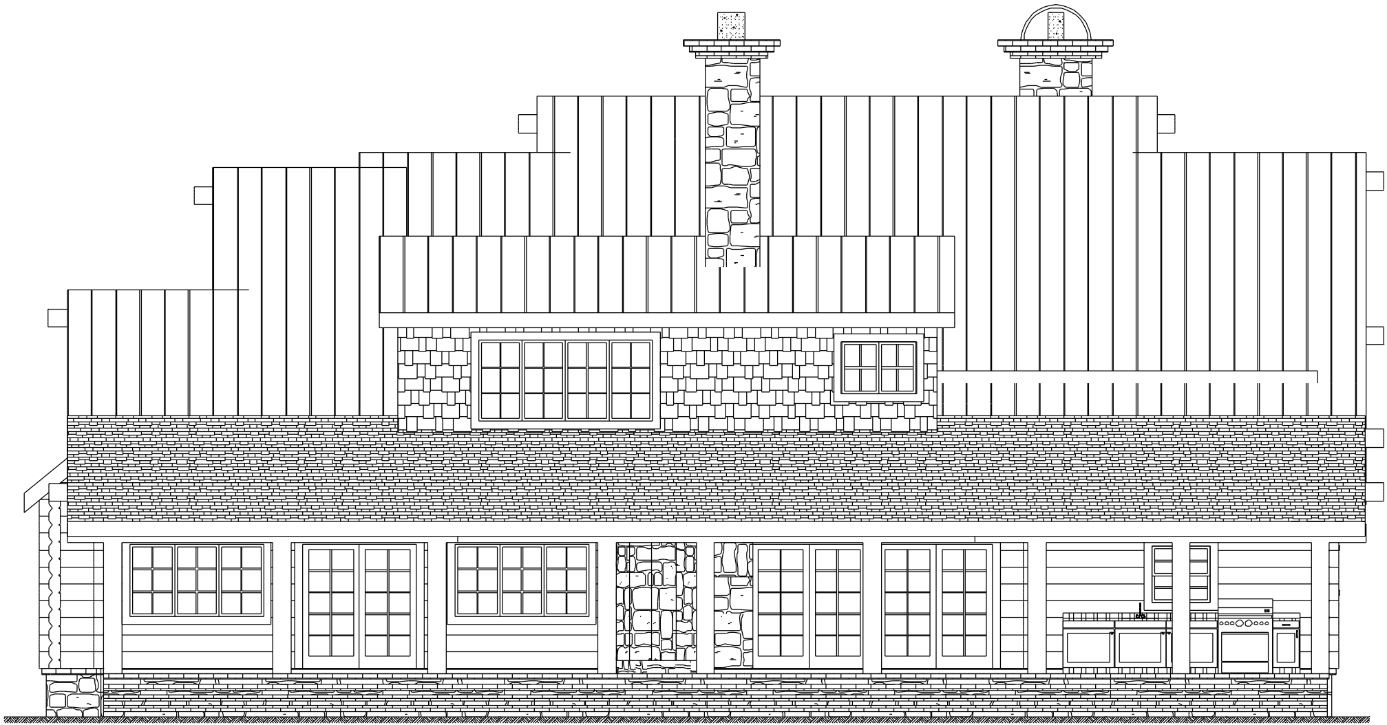
REAR ELEVATION
